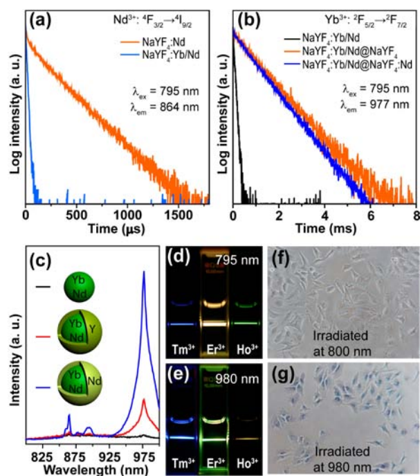
Figure 4. (a) \text{Nd}^{3+} decay curves recorded for \text{NaYF}_4:\text{Nd}(1\%) nanoparticles with and without \text{Yb}^{3+}(30\%) codoping. (b) \text{Yb}^{3+} decay curves recorded for \text{NaYF}_4:\text{Yb}/\text{Nd}(30/1\%) nanoparticles and the corresponding core-shell nanoparticles coated with \text{NaYF}_4 or \text{NaYF}_4:\text{Nd}(20\%) . (c) Near-IR photoluminescence spectra of the nanoparticles shown in (b). (d, e) Luminescence photographs of activator emissions ( \text{Tm}^{3+} 0.5%, \text{Er}^{3+} 0.5%, \text{Ho}^{3+} 1%) for \text{Nd}^{3+} -sensitized and \text{Yb}^{3+} -sensitized nanoparticles under 795 and 980 nm irradiation, respectively (laser power: 100 mW). The same particle concentration for each set of comparisons was obtained by normalizing the particle absorption at 976 nm. (f, g) Optical microscopy images of trypan blue-treated HeLa cells recorded after irradiation for 5 min at 800 and 980 nm, respectively ( 6 \text{ W}/\text{cm}^2 ).
