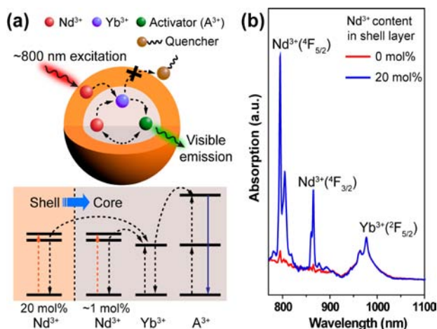
Figure 1. (a) Schematic design (top) and simplified energy level diagram (bottom) of a core–shell nanoparticle for photon upconversion under 800 nm excitation. \text{Nd}^{3+} ions doped in the core and shell layers serve as sensitizers to absorb the excitation energy and subsequently transfer it to \text{Yb}^{3+} ions. After energy migration from the \text{Yb}^{3+} ions to activator ions, activator emission is achieved via the \text{Nd}^{3+} -sensitization process. (b) Near-IR absorption spectra of \text{NaYF}_4:\text{Yb}/\text{Nd}(30/1\%) nanoparticles coated with an inert \text{NaYF}_4 shell or an active \text{NaYF}_4:\text{Nd}(20\%) shell. The absorption spectra were normalized at 976 nm for comparison.
